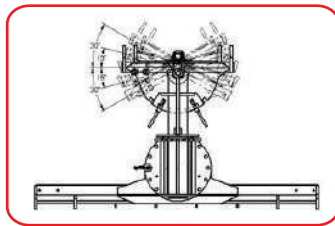
Offset Position
